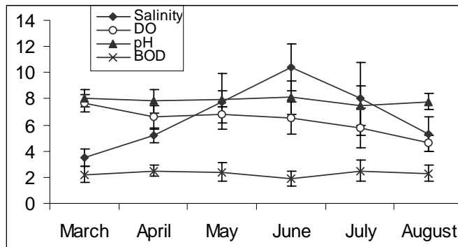
Fig.5.1.4. Changes in physico-chemical parameters of water in 10 shrimp ponds throughout the growing cycle. Values (mean ± SD) are for salinity (ppt), DO (mg/l), BOD (mg/l) and pH.
