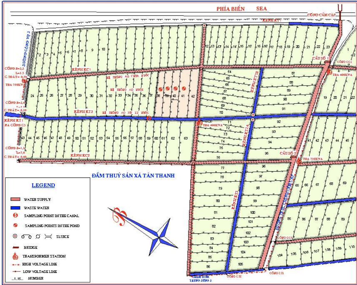
Figure 2.1b: Characteristic of canal system and cultured ponds in Doson -Vietnam
