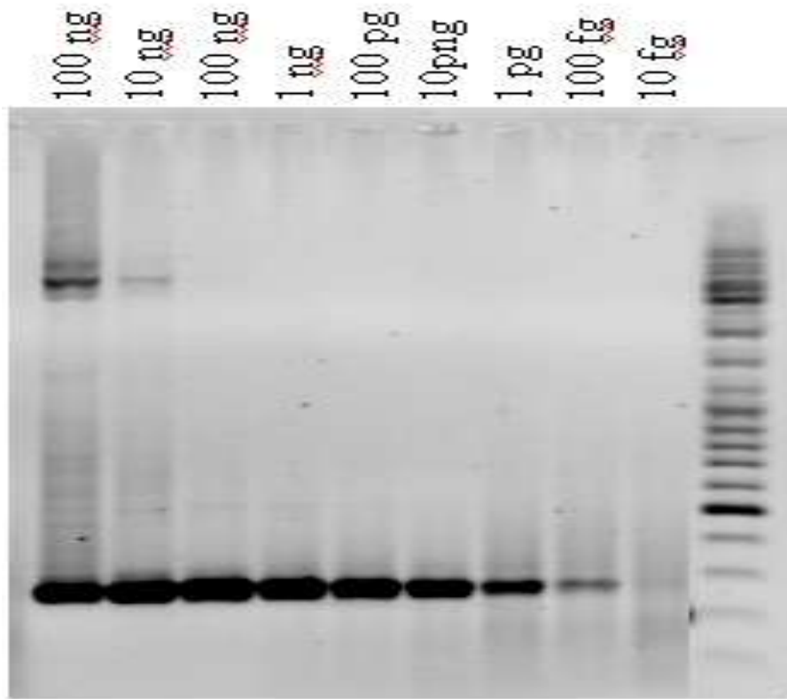
Figure 2. Sensitivity of the competitive PCR assay to detect target DNA.
